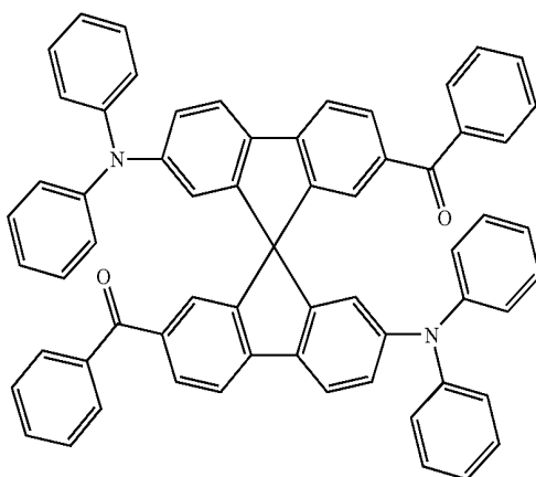
Example 45
