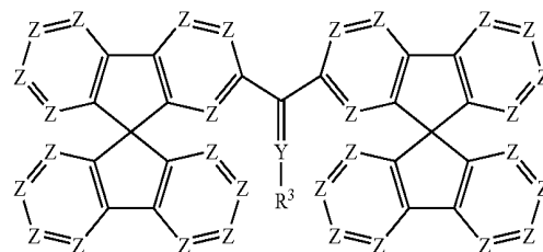
formula (15)
