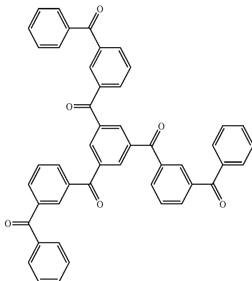
Example 41
