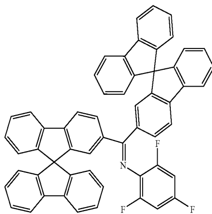
Example 18
