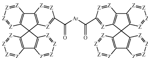
formula (13)
