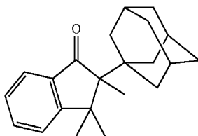
Example 33
