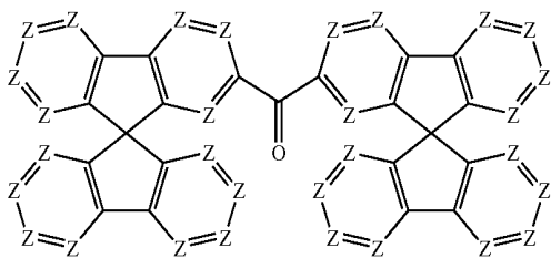
formula (12)
