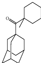
Example 34
