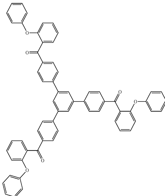
Example 39
