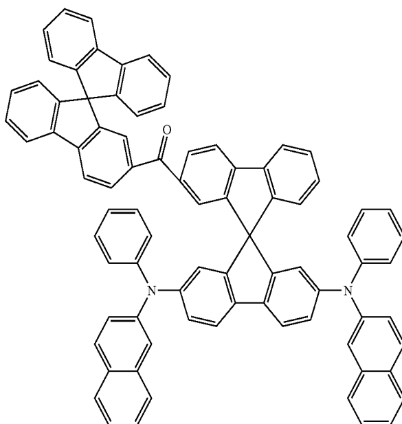
Example 47
