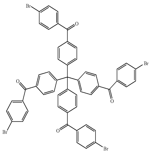
Example 29
