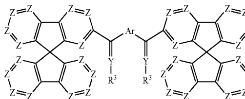
formula (15)
