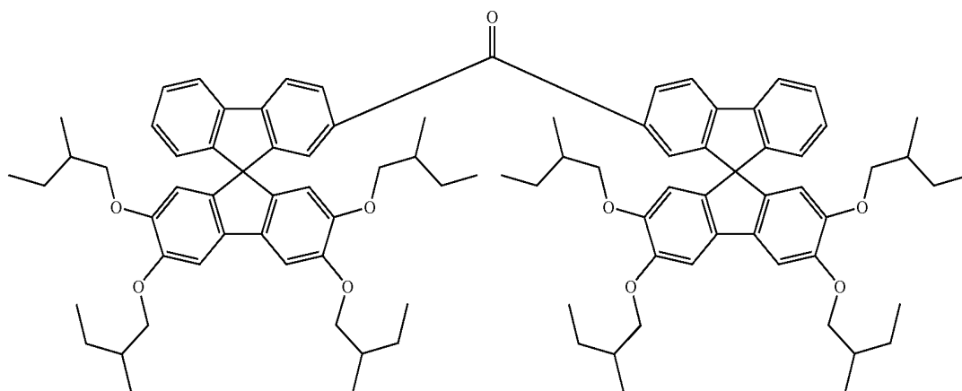
Example 14
