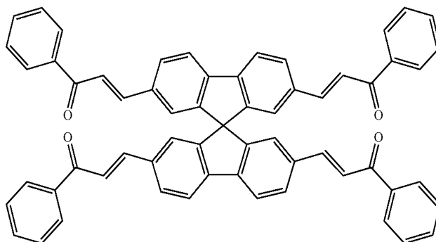
Example 51
