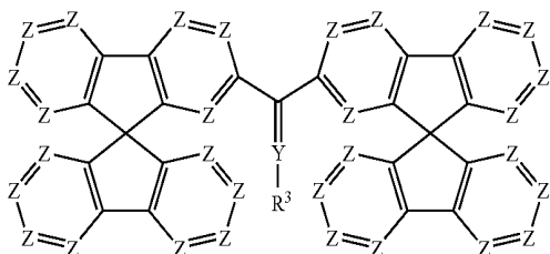
formula (15)
