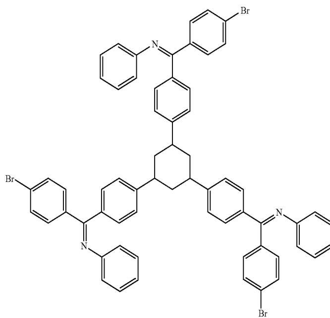
Example 31
