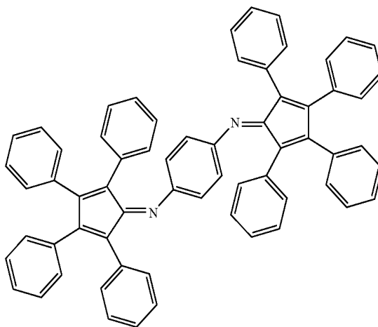
Example 23
