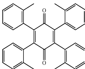
Example 13
