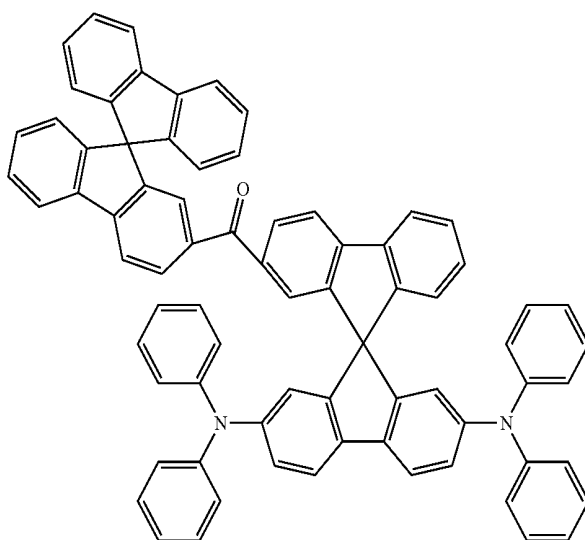
Example 46
