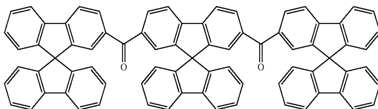
Example 35
