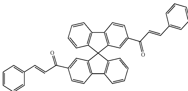
Example 48
