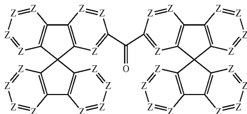
formula (12)
