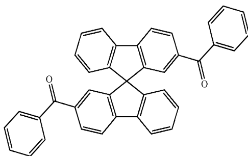
Example 4
