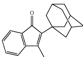
Example 32
