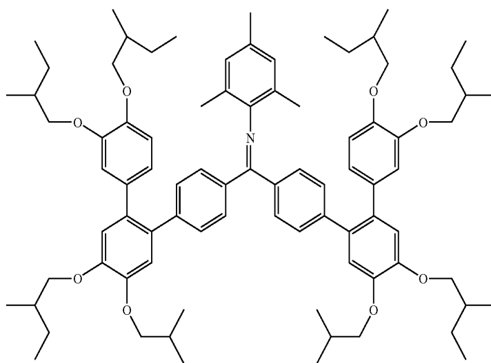
Example 25
