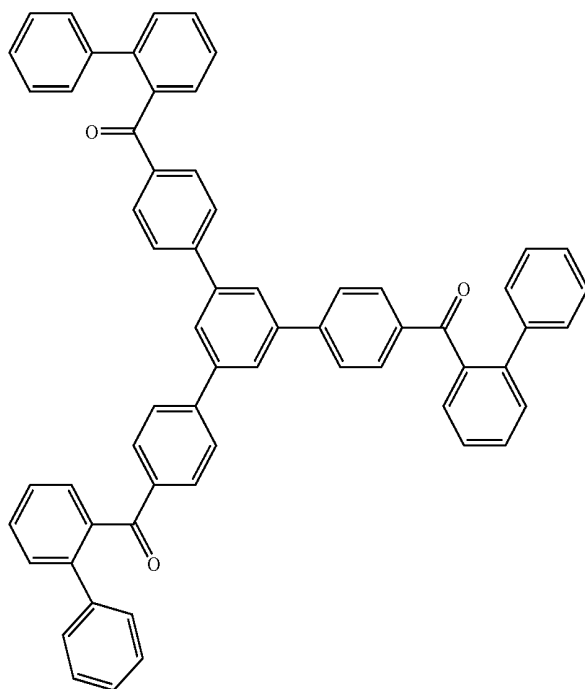
Example 38
