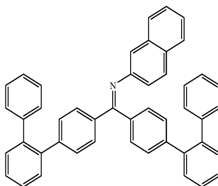
Example 20
