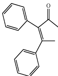
Example 12
