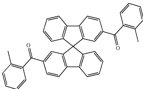
Example 5
