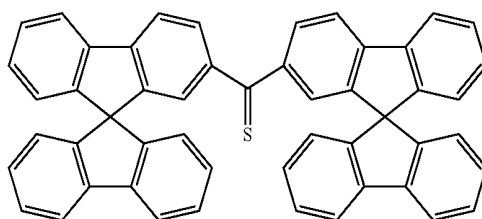
Example 16
