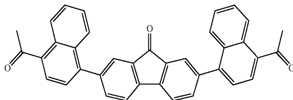
Example 10
