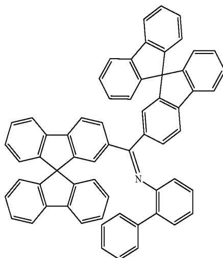
Example 19
