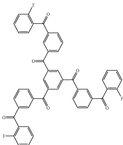
Example 42
