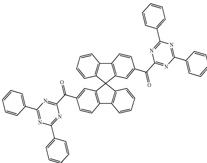
Example 8
