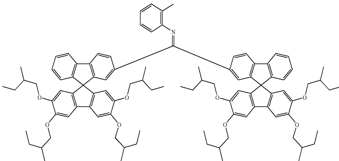
Example 22
