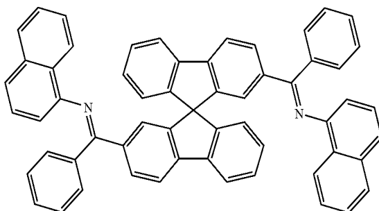
Example 21
