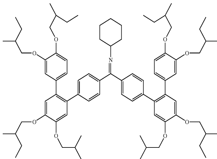
Example 24
