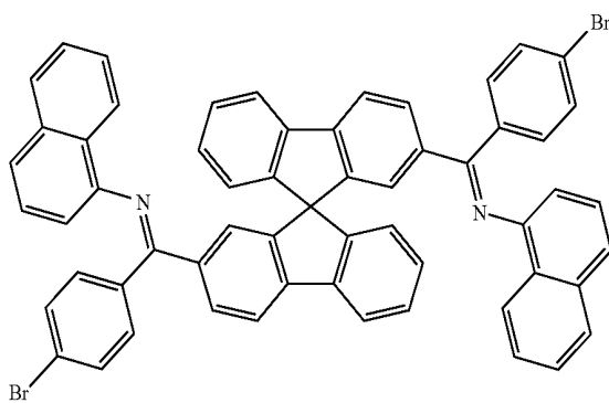
Example 28
