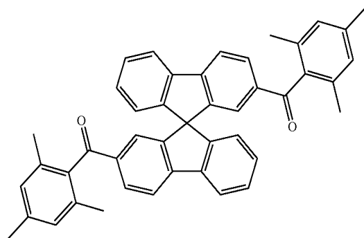
Example 6
