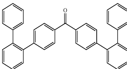
Example 11
