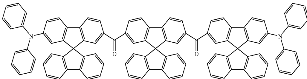
Example 44
