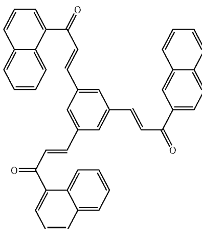
Example 50
