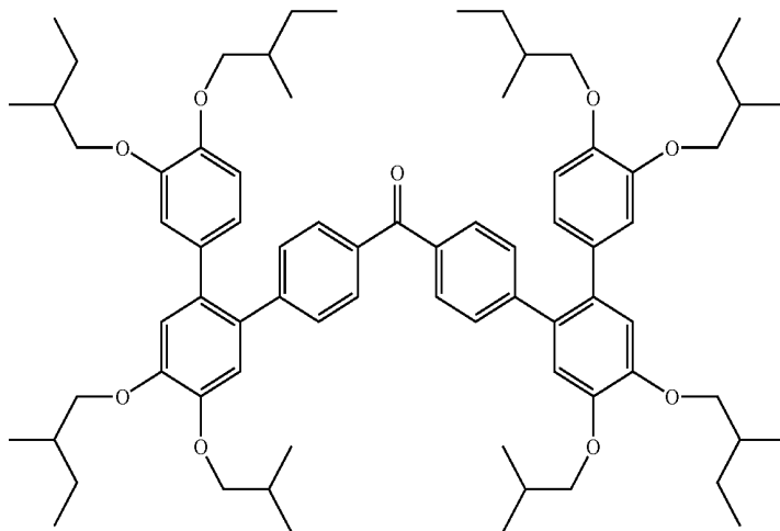
Example 15
