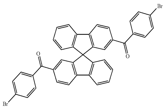
Example 26
