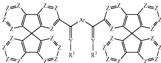
formula (15)
