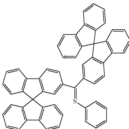
Example 17
