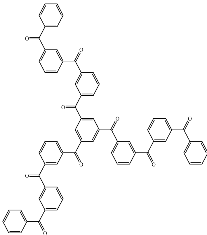
Example 43
