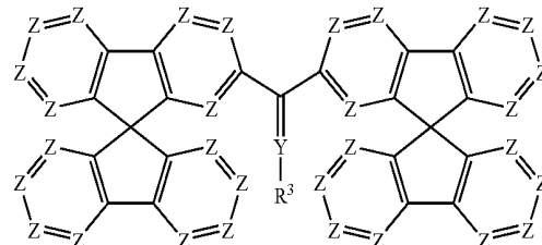
formula (15)
