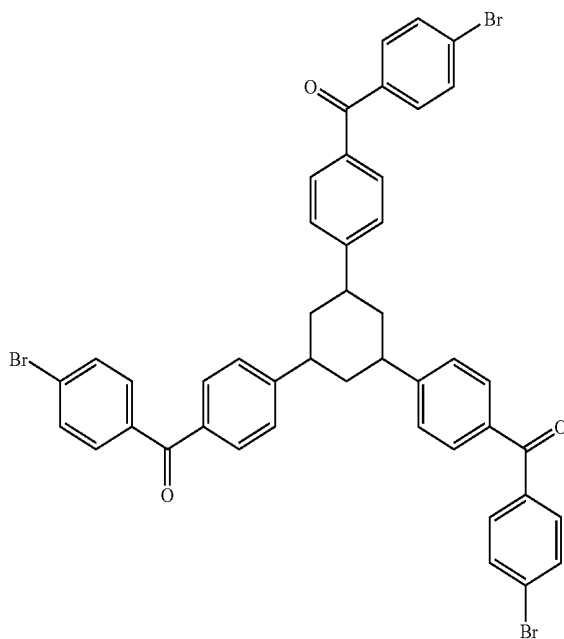
Example 30
