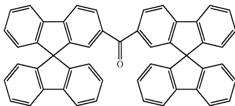
Example 1
